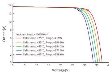
Current-Voltage Curve
